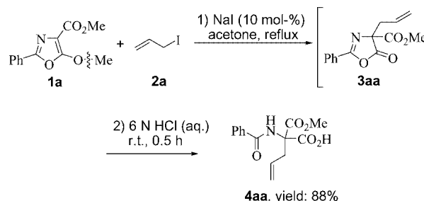
Scheme 3. Tandem allylation/ring-opening reaction of 1a with 2a to form 4aa .
