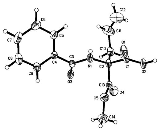
Figure 1. ORTEP representation of compound 4aa .
