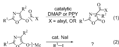
Scheme 1. Two routes for the synthesis of azalactones by C–O bond cleavage.
